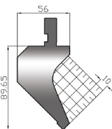
Full Gooseneck Punch (P120)
