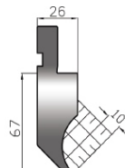
Semi Gooseneck Punch (P97)
